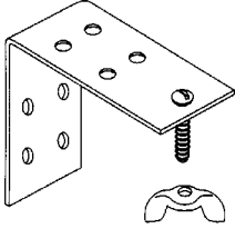
New York Style Bracket Outside Bracket 2" H x 1 7/8" D x 1" W RWC-60025
